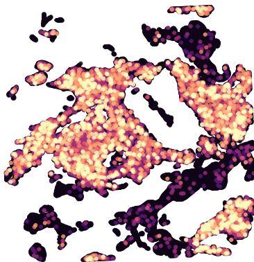
obj2 - H&E
